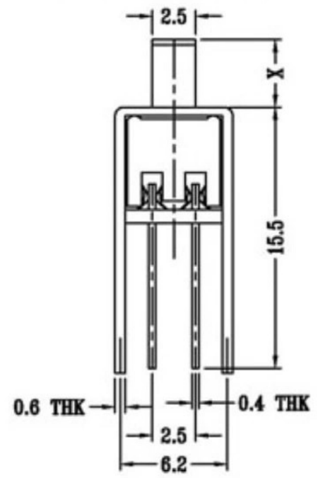
SCHEMATIC (SHORTING)
