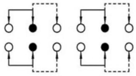
SCHEMATIC (SHORTING)
