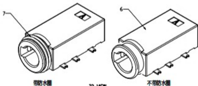
3D VIEW
