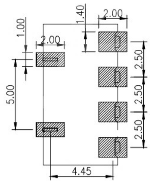
RECOMMENDED PCB LAYOUT TOP VIEW (.XX±0.05)
