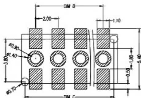
RECOMMENDED PCB LAYOUT TOL:(<math>\pm 0.05</math>)
