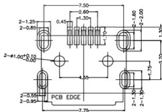
RECOMMENDED PCB LAYOUT TOL:±0.10(TOP VIEW)
