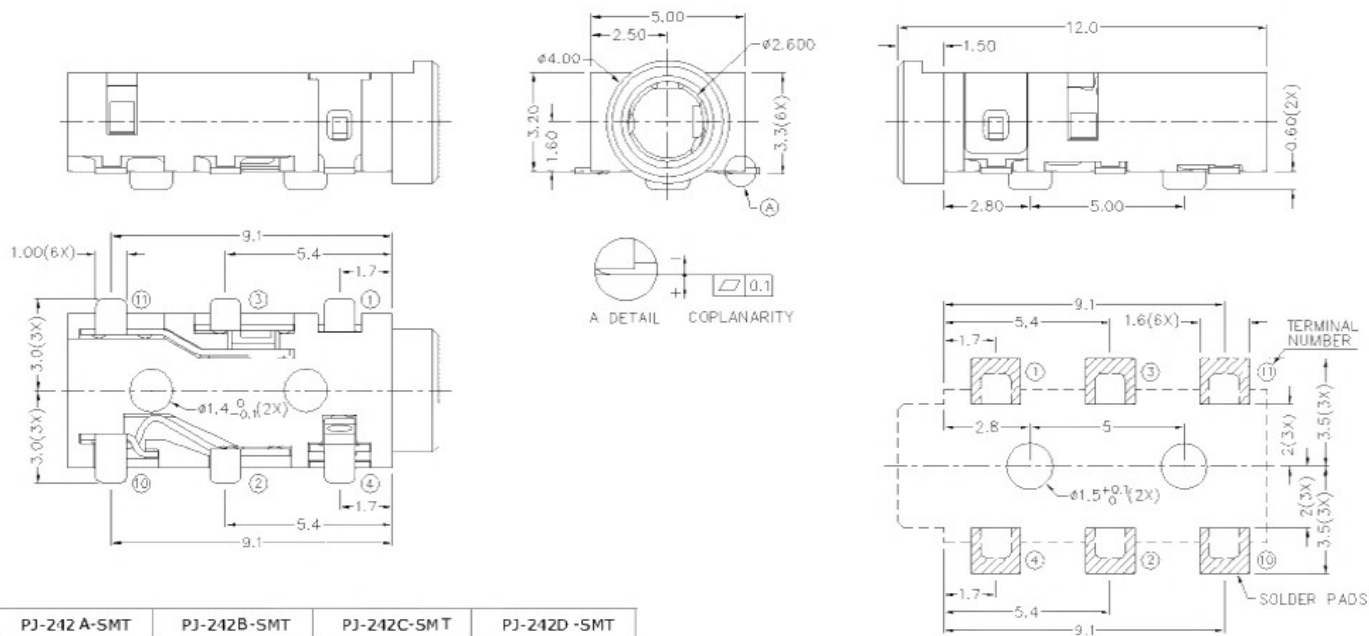
Recommended PCB Layout Top View
