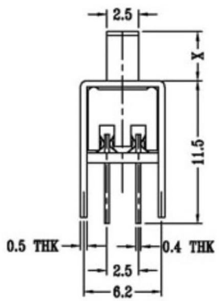
SCHEMATIC (SHORTING)
