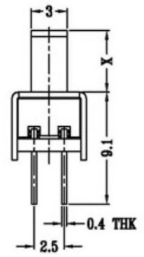
SCHMATIC (SHORTING)
