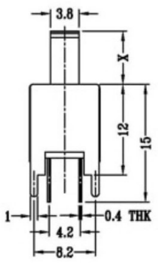
SCHMATIC (SHORTING)
