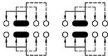
SCHEMATIC (SHORTING)
