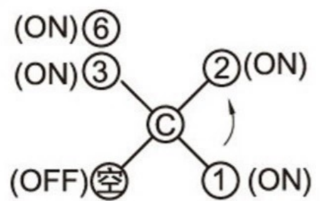
SCHEMATIC (NON-SHORTING)
