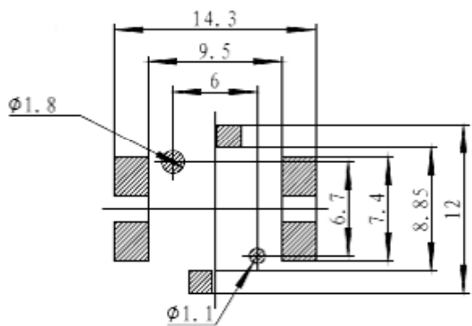
PC board mounting hole dimensions (Viewed from the direction A)
