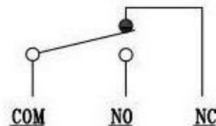
SCHEMATIC (NON-SHORTING)
