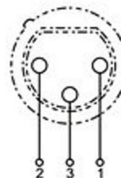
SCHEMATIC LAYOUT
