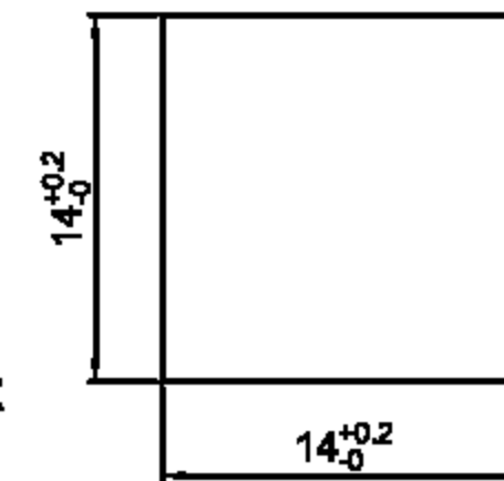
PANEL HOLE
