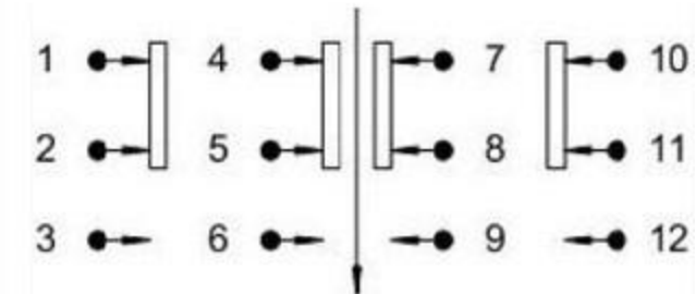
SCHEMATIC (NON-SHORTING)
