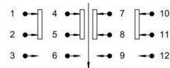
SCHEMATIC (NON-SHORTING)
