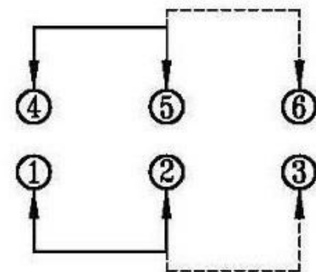
SCHEMATIC (NON-SHORTING)
