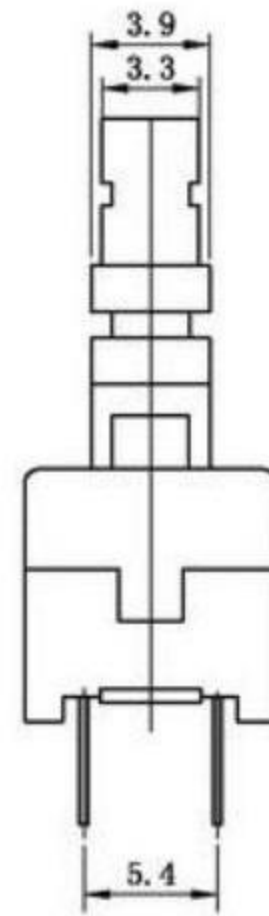
SCHEMATIC
