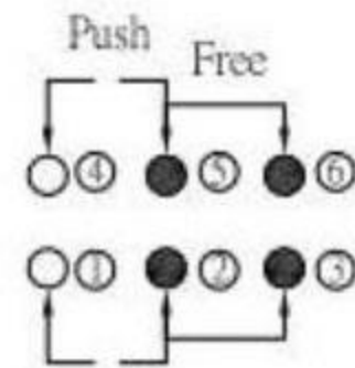
SCHEMATIC (NON-SHORTING)
