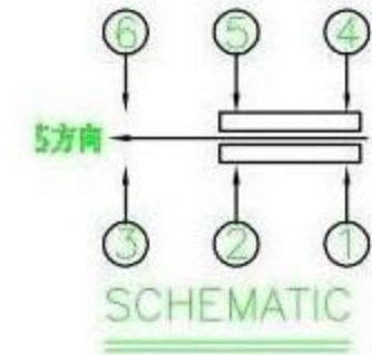
SCHEMATIC (NON-SHORTING)
