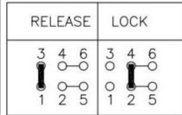
SCHEMATIC (NON-SHORTING)
