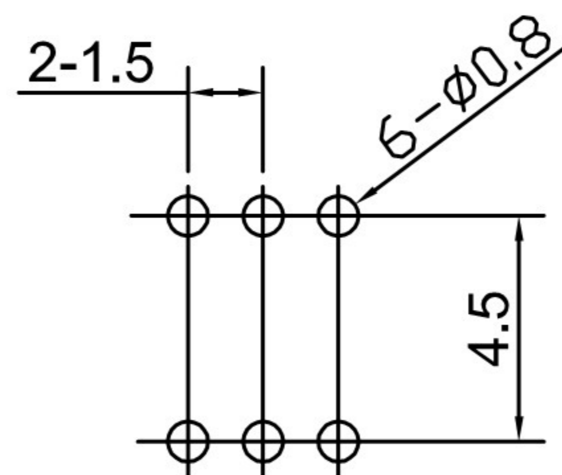
P. C. B LAYOUT
