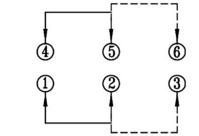
SCHEMATIC (NON-SHORTING)
