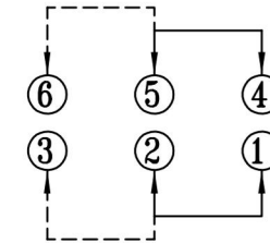
SCHEMATIC (NON-SHORTING)
