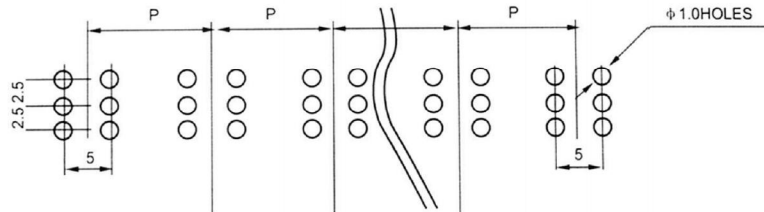
PCB LAYOUT
