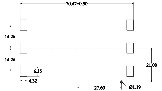
PCB LAYOUT
