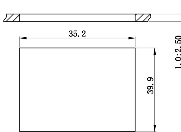
PANEL CUT-OUT
