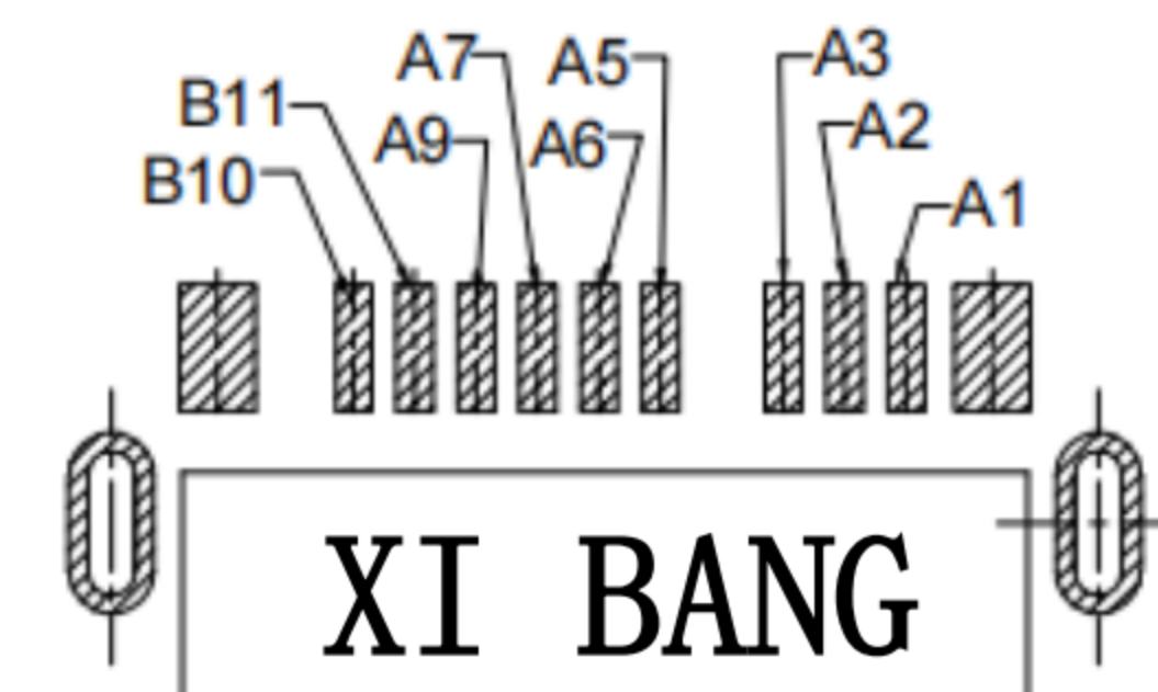
PIN DIGIT DIAGRAM
