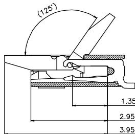
SECTION A-A(2:1)
