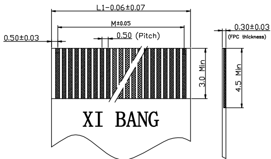
适用FPC尺寸 APPLICABLE FPC
